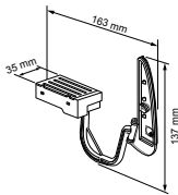
262 085 White base - Clear shark foot
