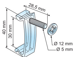
262 545 Clear - For electronic rail
