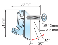
262 645 Coupon-holder clip P25
