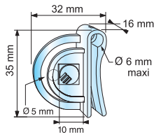
262 047 Clear - for wire and divider
