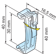
262 543 Clear - for electronic labelling rail
