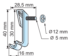
262 045 Coupon-holder clip for 30 to 40 mm label-holder
