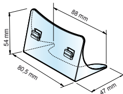
797 331 Leaflet dispenser leg
