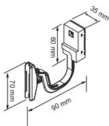
841 207 White base - Clear frame clips
