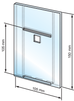
124 105 Rectangle format 105widthx150Htmm
