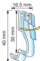
262 043 Clear - for electronic labelling rail
