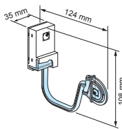
262 841 White base - Clear shelf clips
